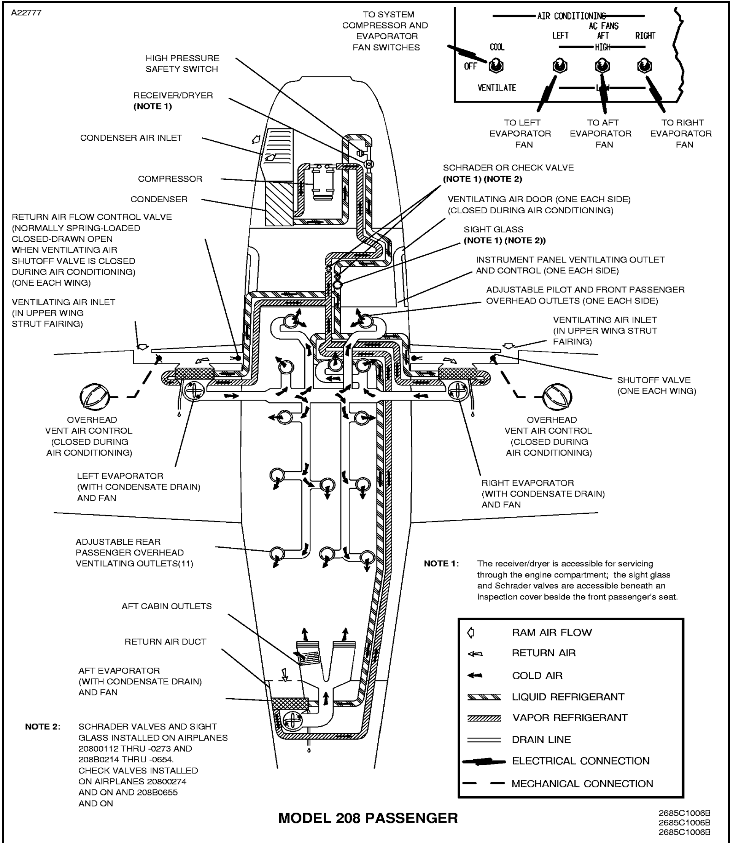
Figure 1 : Sheet 2 : Air Conditioning System Schematic
