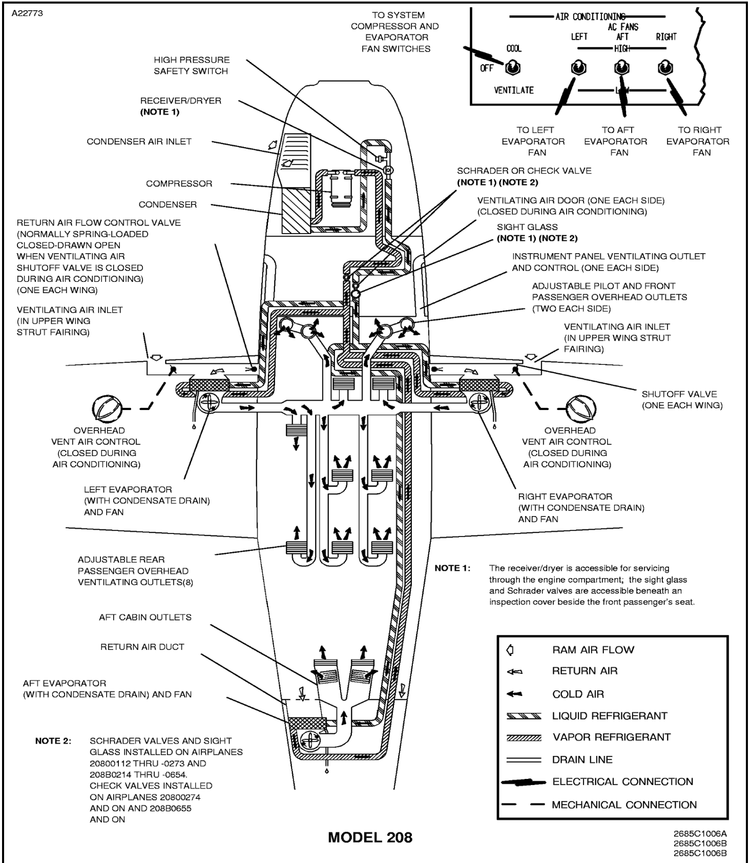
Figure 1 : Sheet 1 : Air Conditioning System Schematic
